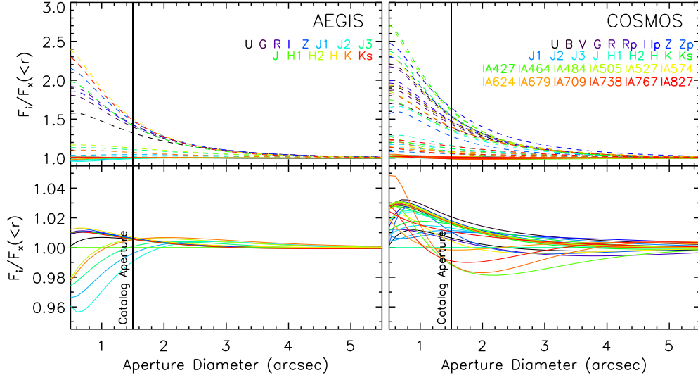
FIG. 6.— The ratio of the growth curve for all optical to NIR bands F_i relative to the band with the worst seeing F_x (where x = H_1 in AEGIS and H_2 in COSMOS). The top panel shows the ratio before convolution (dashed lines) and the bottom panel shows after convolution (solid lines). Note the different y-axis scales of the top and bottom panels. The PSF matched images have accurate colors to < 2\% for the catalog aperture diameter of 1.5'' .
