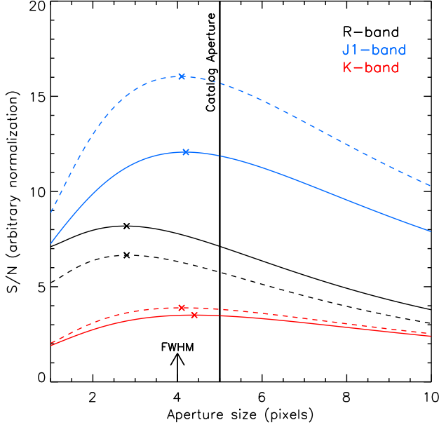
FIG. 7.— The signal-to-noise as a function of the aperture size, derived from the ratio of the growth curve and the noise properties for the R (black), J_1 (blue) and K -band images (red). The solid lines are for the COSMOS field and the dashed lines are for AEGIS, with an “x” marking the peak in S/N. The FWHM of the PSF matched K -band image is shown with an arrow. We use an aperture diameter of 5 pixels ( 1.5'' ) when creating the NMBS catalogs so as to optimize the S/N while remaining larger than the FWHM.
