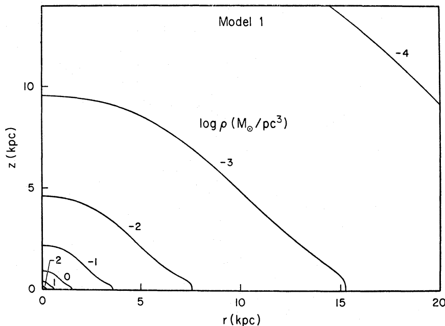
FIG. 1. Contours of constant stellar density \rho in one quadrant of a meridional plane of Model 1; curves are labelled with the logarithm of the stellar density in units of M_\odot \text{pc}^{-3} . This model is similar to Model 4 of Paper III except that the boundary radius is 100 kpc instead of 30 kpc.
