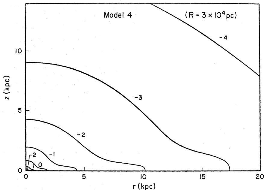
FIG. 4. Density contours for Model 4, in which star formation is tidally inhibited in accordance with equation (3) with B = 0.25 .
