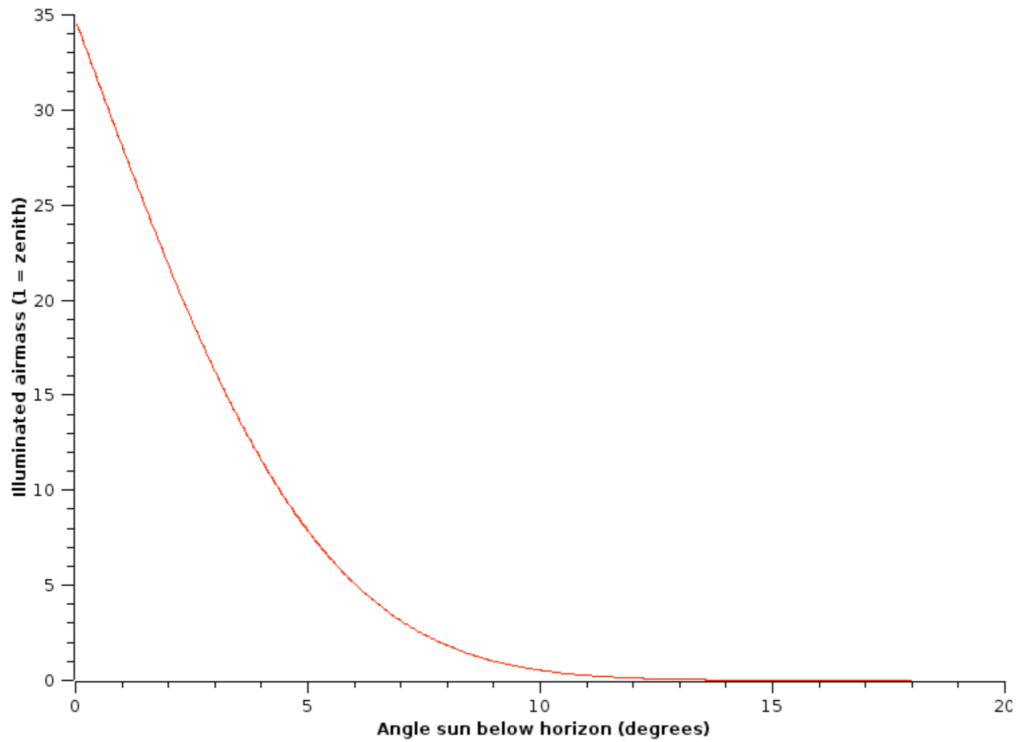
Amount of air that is lit after sunset at the horizon
