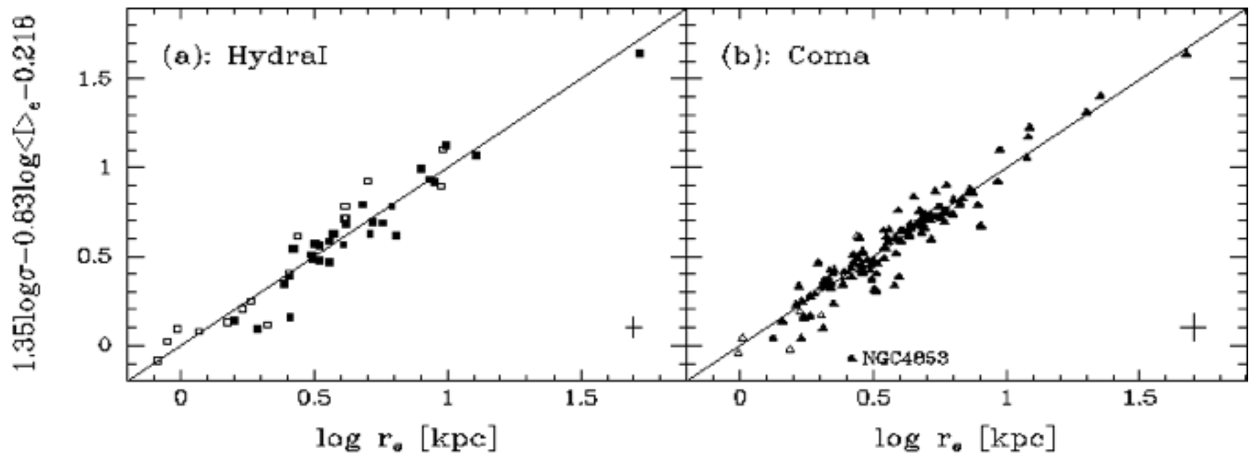
Figure 7.3: The Fundamental Plane in Coma, Ell (7.7) galaxies on a plane, Data symbols as in Fig. 7.1. called "Fundamental Plane"
