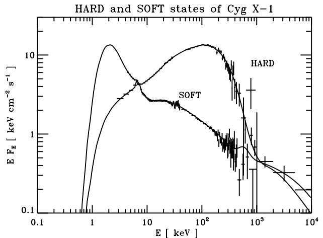
Figure 1: Best fits to the two spectral states of Cyg X-1 using the hybrid thermal/non-thermal pair model. The hard state data are simultaneous observations by Ginga, OSSE, and COMPTEL (June 1991). The best fit model has the following parameters l_{nth} = 1.3 , l_s = 1 (frozen), l_{th} = 11 , \tau_p = 1.47 , T_{bb} = 0.13 keV (f), and Compton reflection amplitude R = 0.3 , give a \chi^2/\text{dof}=56/78 . The soft state data are from the XTE/PCA and OSSE (June 1996). The model spectrum corresponds to the fit parameters: l_{nth} = 5 (f), l_s = 34 , l_{th} = 3 , \tau_p = 0.23 (f), T_{bb} = 0.39 keV, R = 1.1 , giving a \chi^2/\text{dof}=180/169 . In both cases the power-law index for non-thermal electron injection was fixed at \Gamma_{inj} = 2.4 . Spectra cut off at low energies due to interstellar absorption with column density N_H = 0.6 \cdot 10^{22} \text{ cm}^{-2} .
