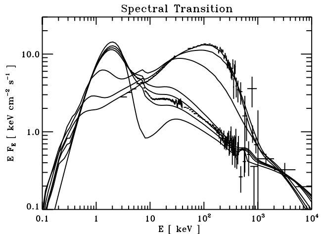
Figure 2: Simulations of the spectral transitions by the HPM. The starting point is the best fit to the hard state data ( r = 6 ). Using the simple scaling laws (see § 4) for l_s, l_{th}, l_{nth} , we obtain the sequence of spectra covering the transition between the hard and soft states as a function of the inner disk radius, r . From top to bottom (at 100 keV), the curves correspond to the inner disk radius of 6, 4, 2, 1.2, 1.15, 1.1, 1.0, respectively. The spectra at r \sim 1.1 - 1.15 are quite close to the observed soft state spectrum.
